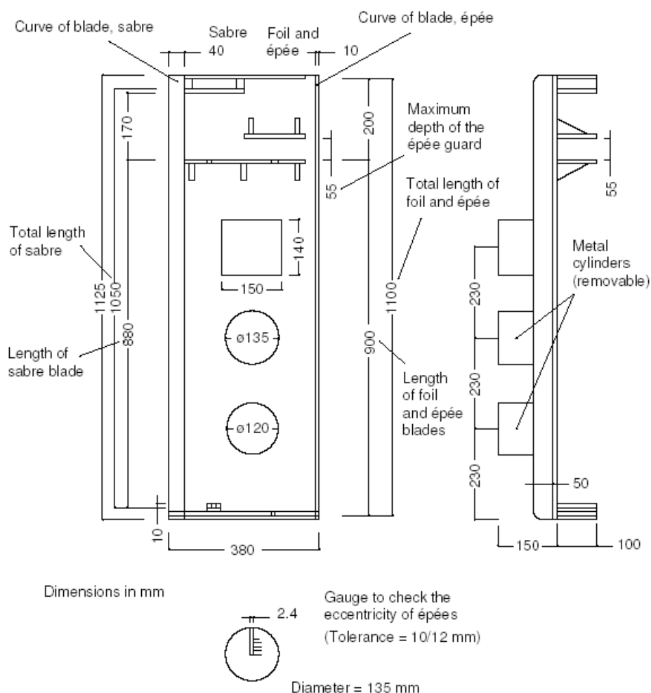
Figure 16. Gauge for checking weapons
