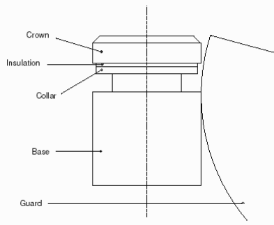
Figure 10. Epée: details of tip of point
