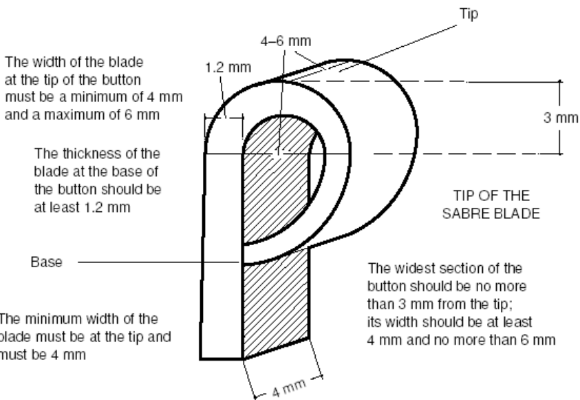
Figure 12. Sabre dimensions and flexibility
