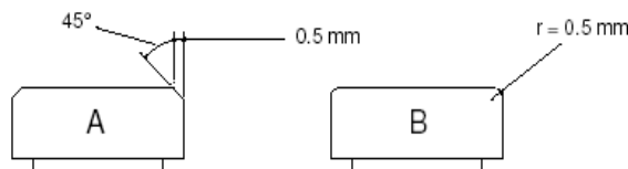
Figure 11. Epée: details of tip of point
